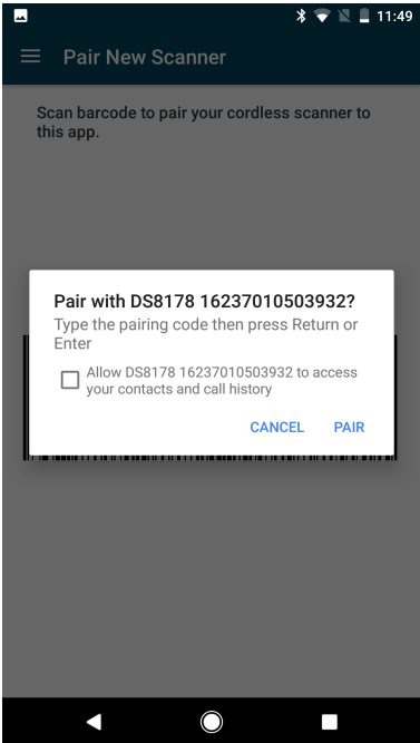
Figure 1-5 Pairing Confirmation
