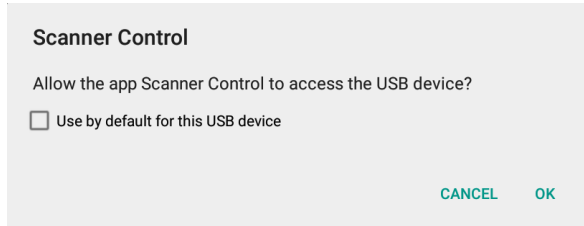
Figure 1-9 Application Permission
