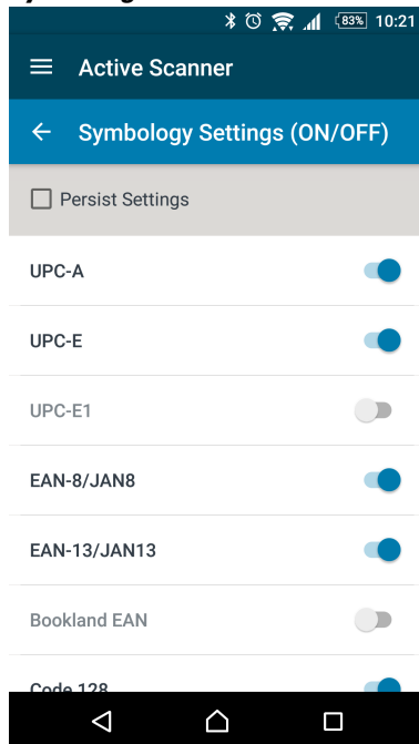
Figure 1-13 Symbology Settings
